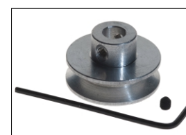
Part No. 918D2. Pulley. 2mm I.D. (25mm dia. x 14.75mm) (Aluminium). 12g Part No. 918D2/1. Pulley 4mm I.D. (25mm dia. x 14.75mm) (Aluminium). 12g
